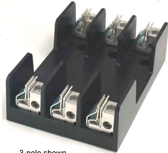
3-pole shown
